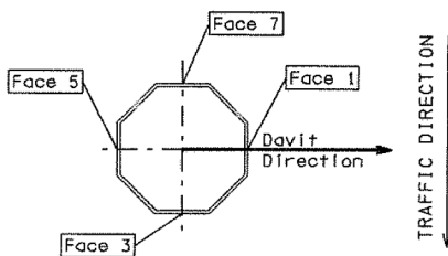
SINGLE DAVIT POLE ORIENTATION.
