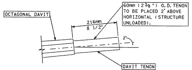
DAVIT TENON DETAILS
