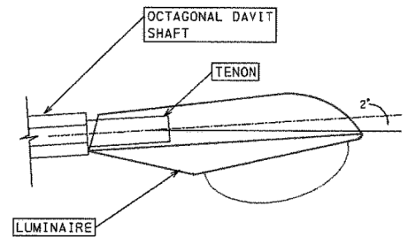
LUMINAIRE INSTALLATION
