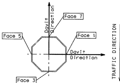
DOUBLE DAVIT 90° POLE ORIENTATION.
