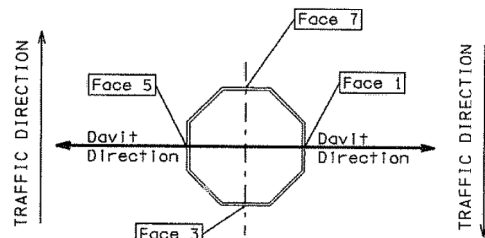
DOUBLE DAVIT POLE ORIENTATION.
