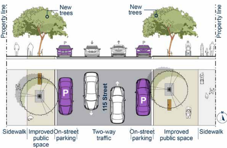
View 1: Proposed
