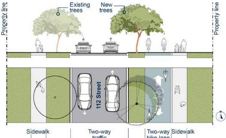
View 4: Proposed
