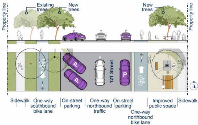
View 2: Proposed
