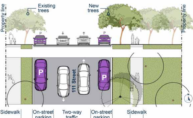
View 2: Proposed
