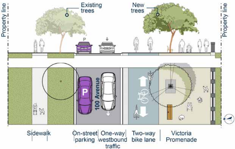
View 3: Proposed
