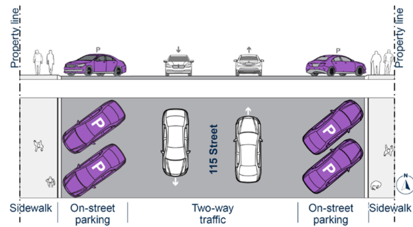
View 1: Existing
