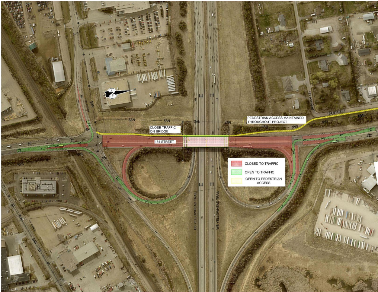
Image 1 - Construction limits
