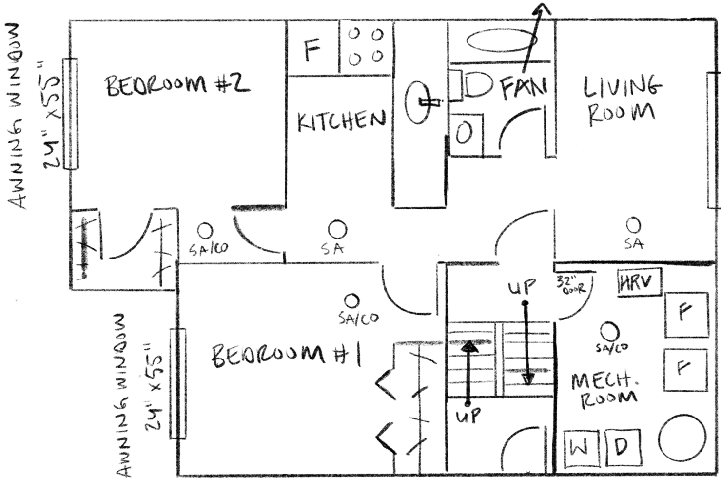
4928-48 STREET BASEMENT PLAN (1170 SQ.FT)
