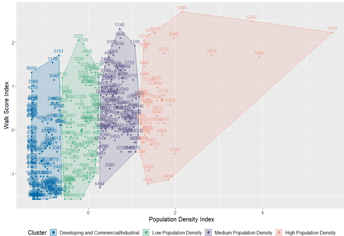
Figure 3-9 Visualization of Neighbourhood Clusters
