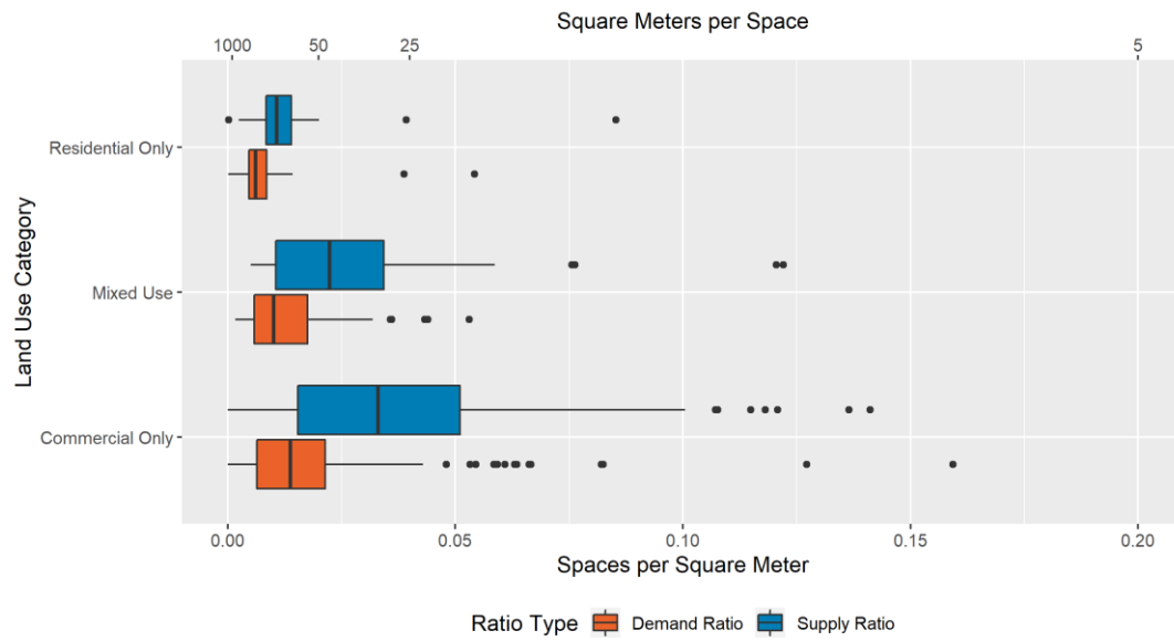
Figure 3-34 Ratio Boxplot, by Overall Land Use
