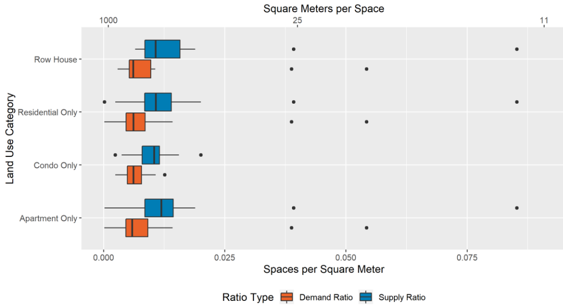
Figure 3-32 Ratio Boxplot, by Residential Land Use
