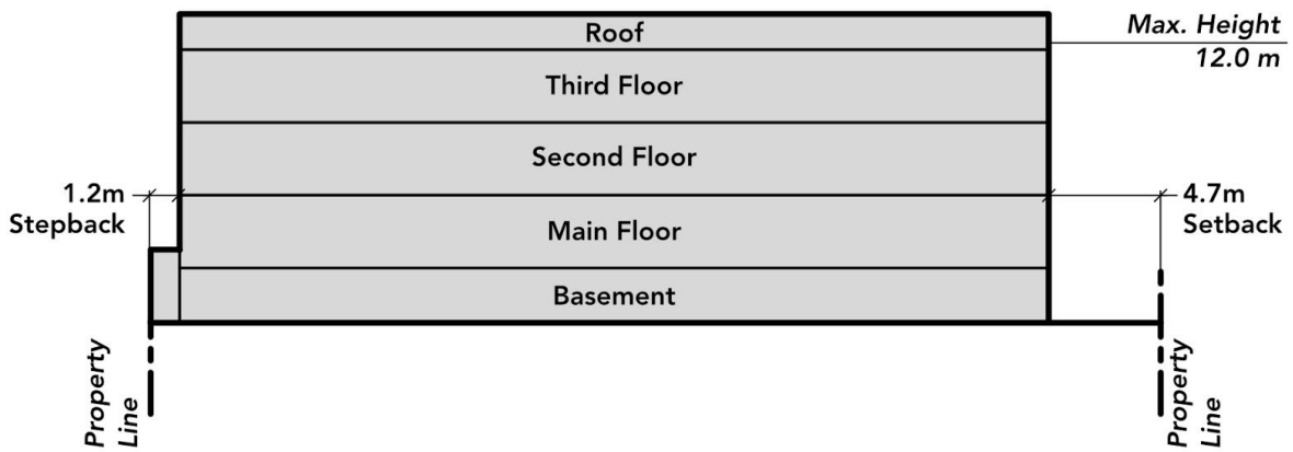
East Elevation
