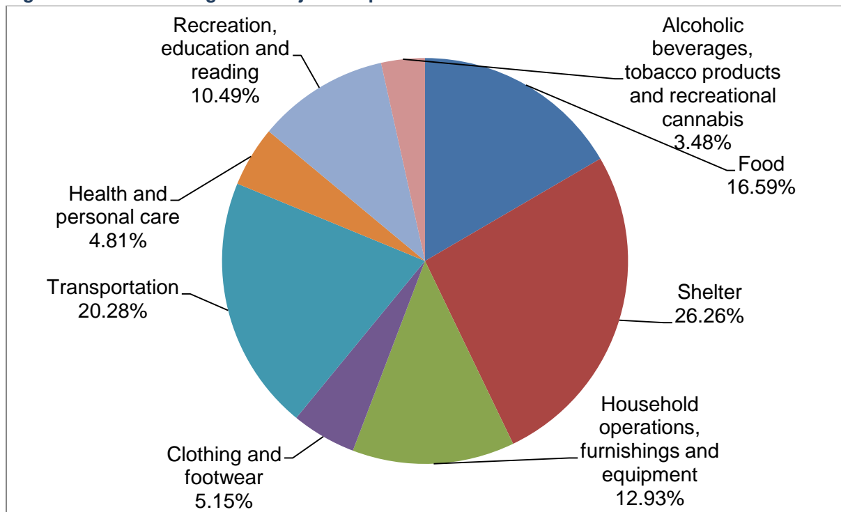
Figure 1: 2017 CPI Weights of Major Components – Alberta
