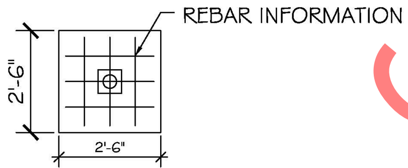
CONCRETE PAD DETAIL
