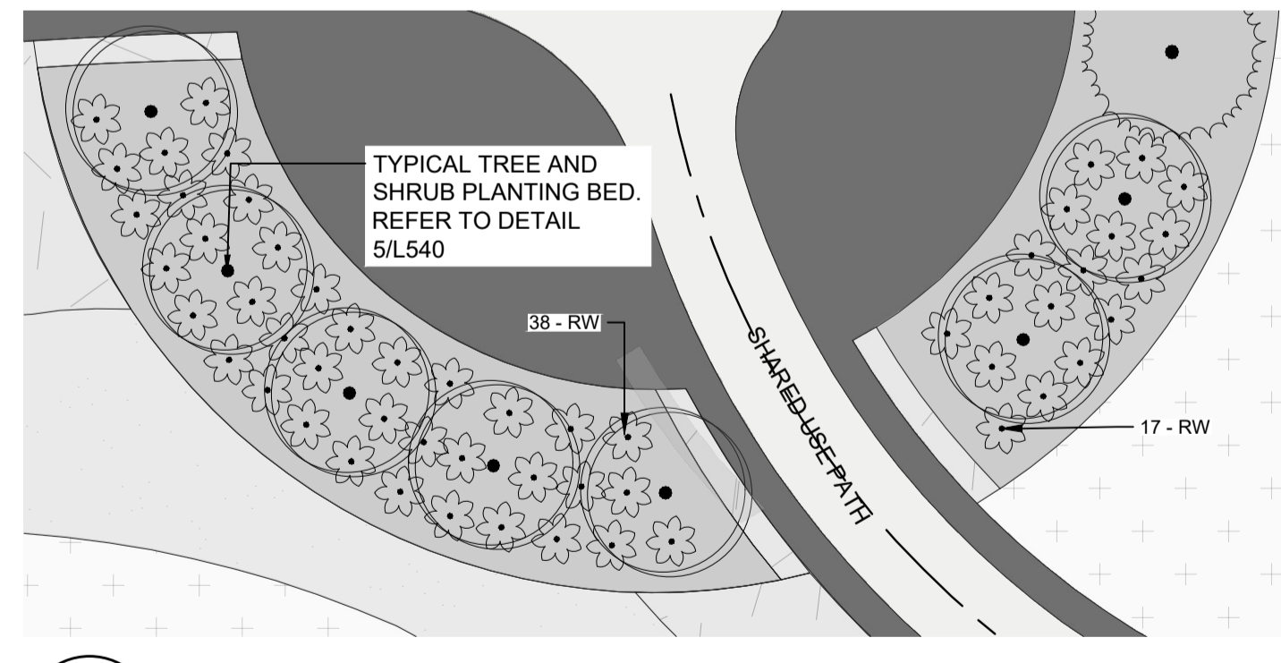
2 CIRCULAR PLAZA PLANT BED ENLARGEMENT L210 1:10
