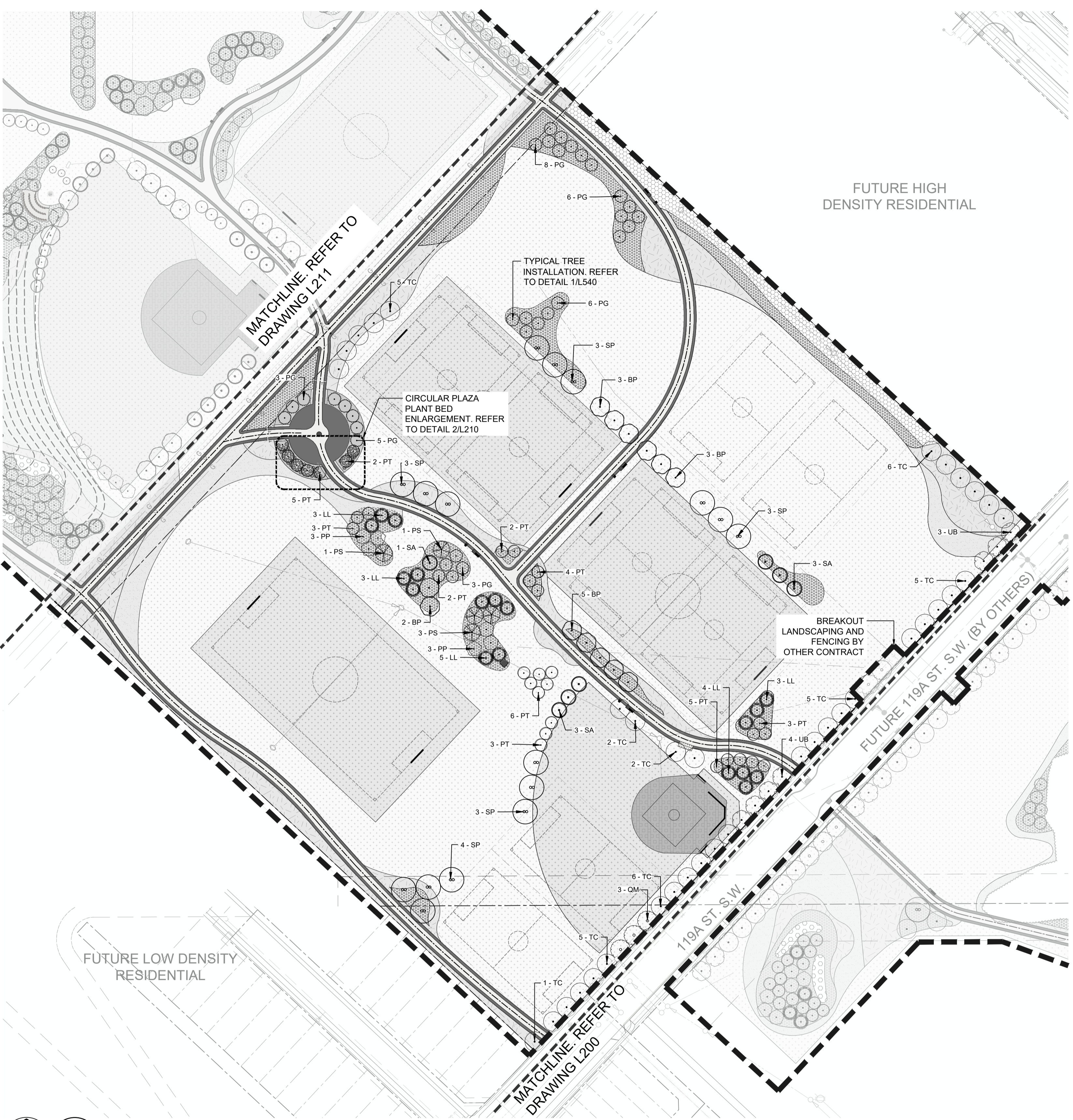
1 STAGE 2A SOUTH PLANTING PLAN L210
