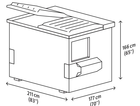
6 Cubic Yard (yd 3 ) Bin
