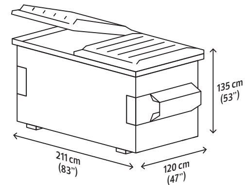
3 Cubic Yard (yd 3 ) Bin
