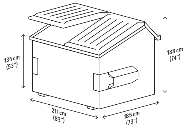
6 Cubic Yard (yd 3 ) Bin (Slant)
