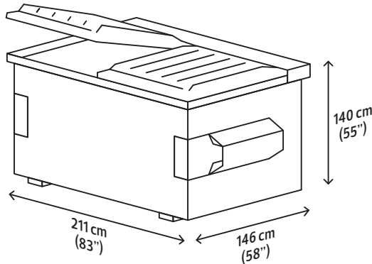
4 Cubic Yard (yd 3 ) Bin
