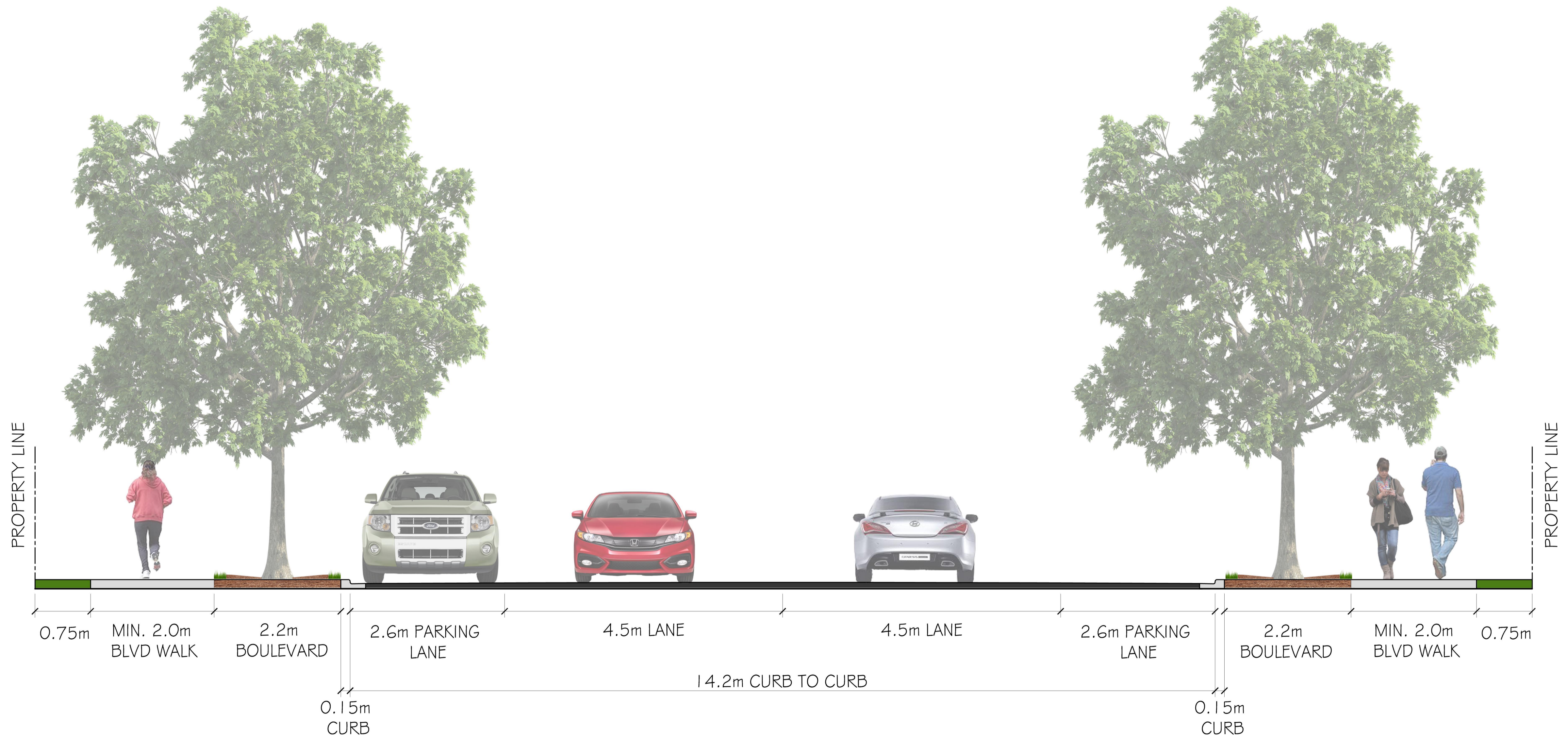
112 STREET PROPOSED IMPROVEMENTS - ELEVATION - LOOKING NORTH
