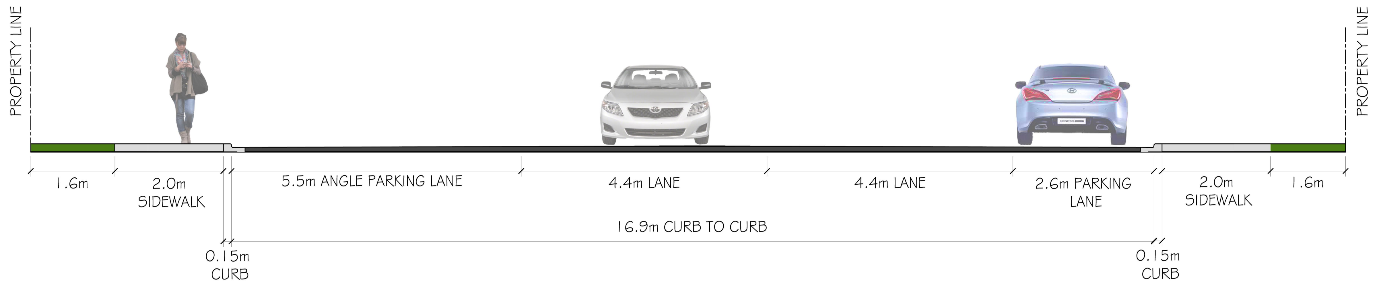
112 STREET QUEEN MARY PARK NEIGHBOURHOOD RENEWAL - ELEVATION - LOOKING NORTH
