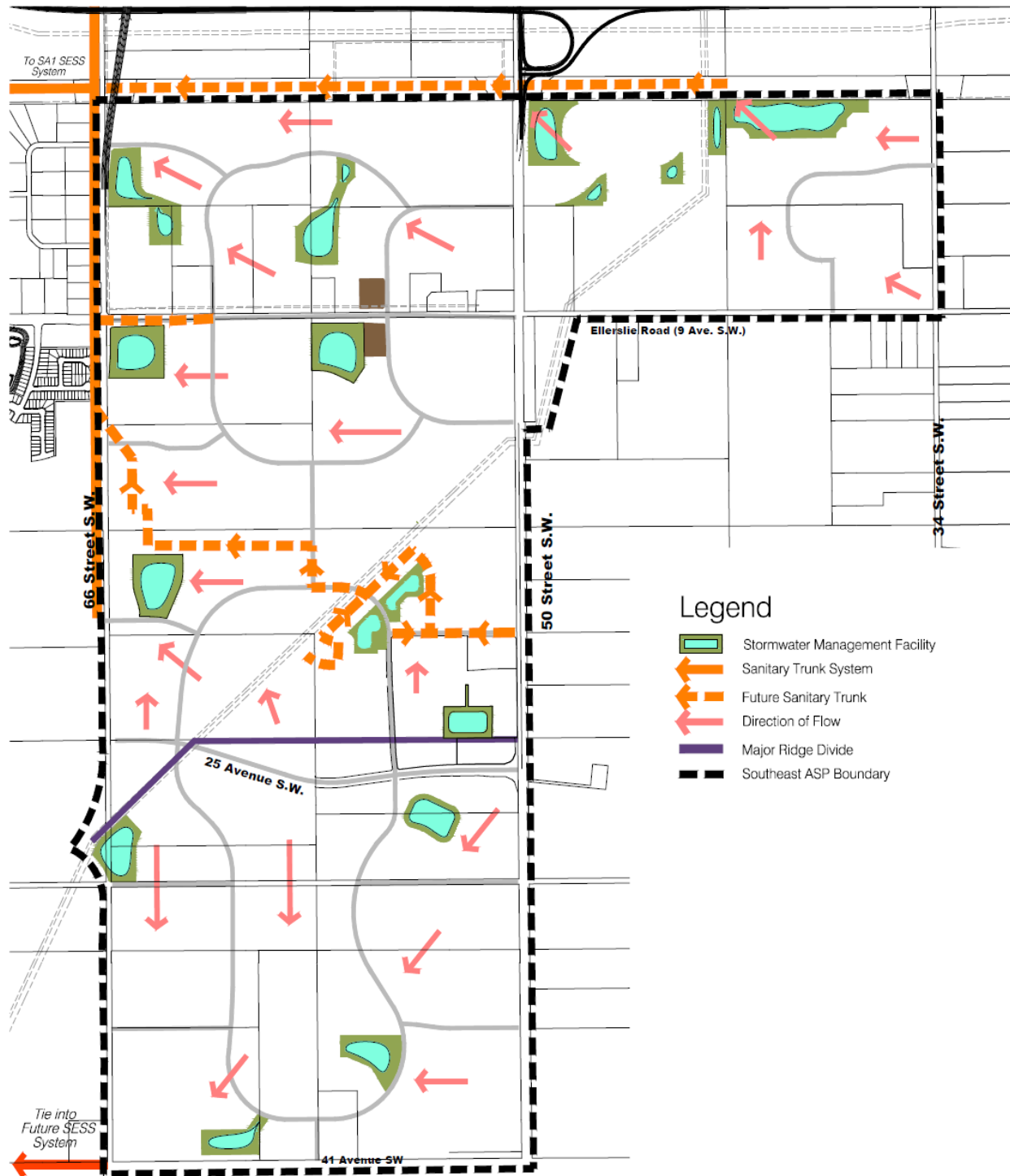
Figure 15.0 – Sanitary System (Bylaw 17676, June 27, 2016)
