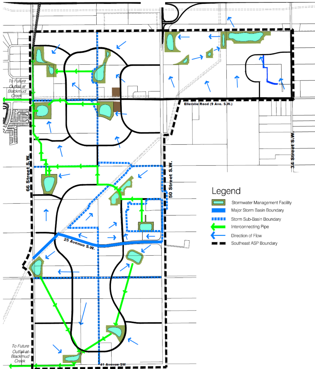
Figure 14.0 – Stormwater System (Bylaw 17676, June 27, 2016)
