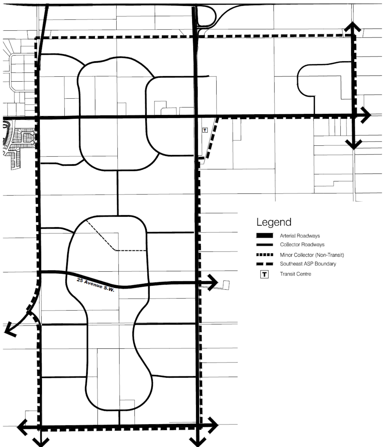
Figure 12.0 – Arterial Roadway Assessment (Bylaw 17676, June 27, 2016)
