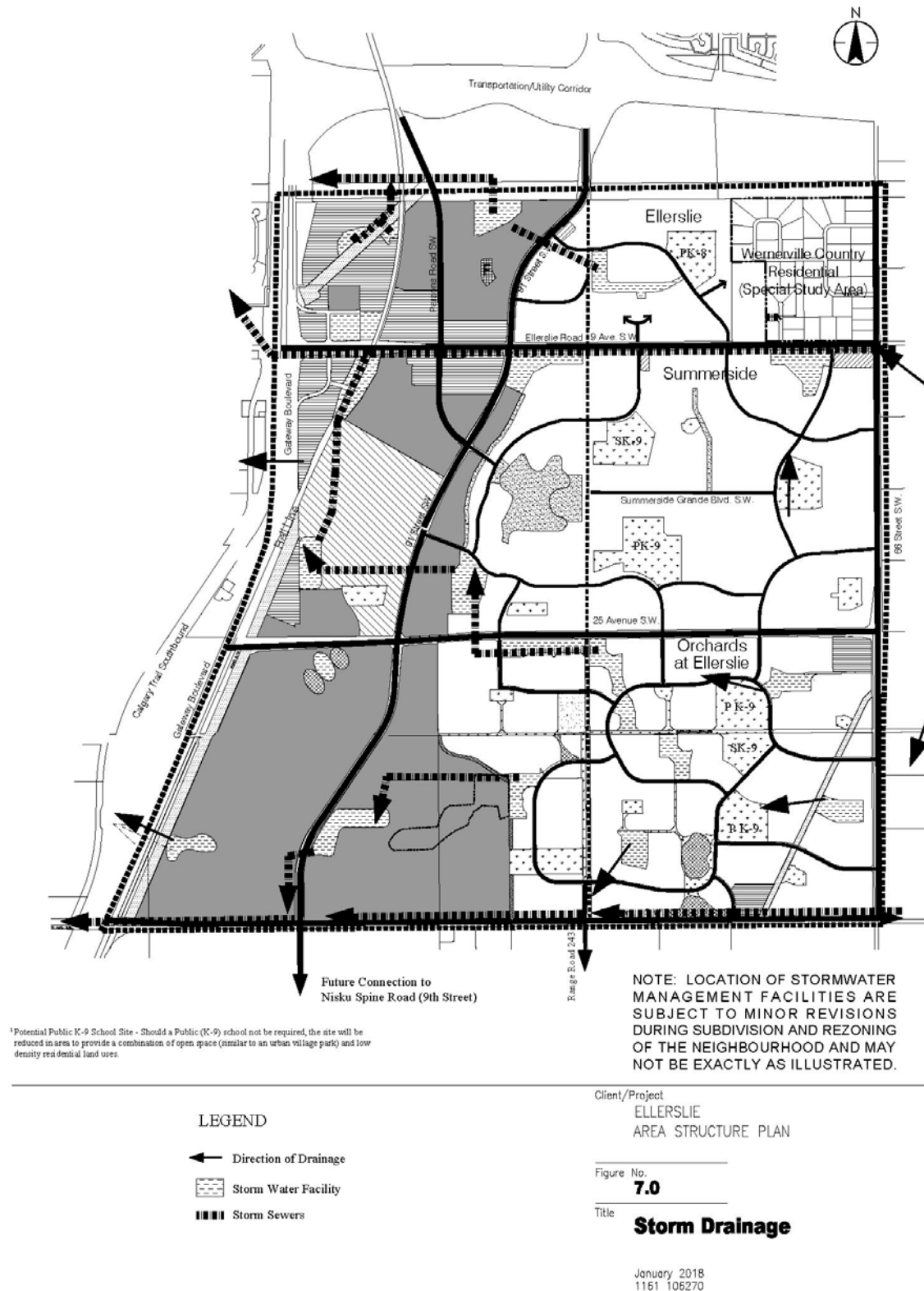
Figure 7 Storm Drainage (As amended by Bylaw 18274, February 12, 2018)
