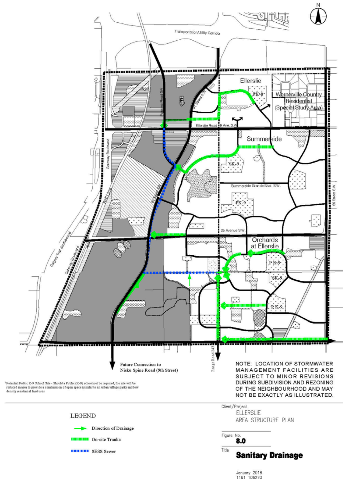
Figure 8 Sanitary Drainage (As amended by Bylaw 18274, February 12, 2018)
