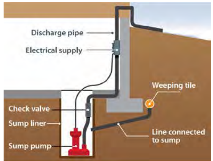
Weeping tile with sump pump. Source: The City of Edmonton, adapted by The City of Calgary
